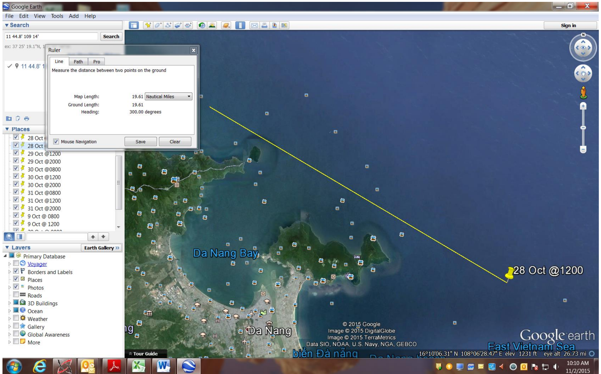
October 28, 1966. Uss Ponchatouls AO-148 refueling USS Vogelgsang DD-862 between 1055 and 1138 steaming at 18 kts on course 120
